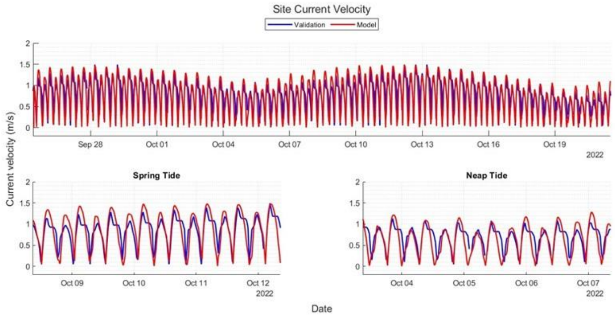
Figure 2-9: Model Current Velocity (m/s) 2022 Validation Data at Station SN011I
