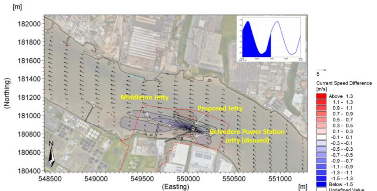
Figure 3-11: Scenario 1 vs. Scenario 3 – Difference in Flow Speed Magnitude at Peak Spring Flood Tide
