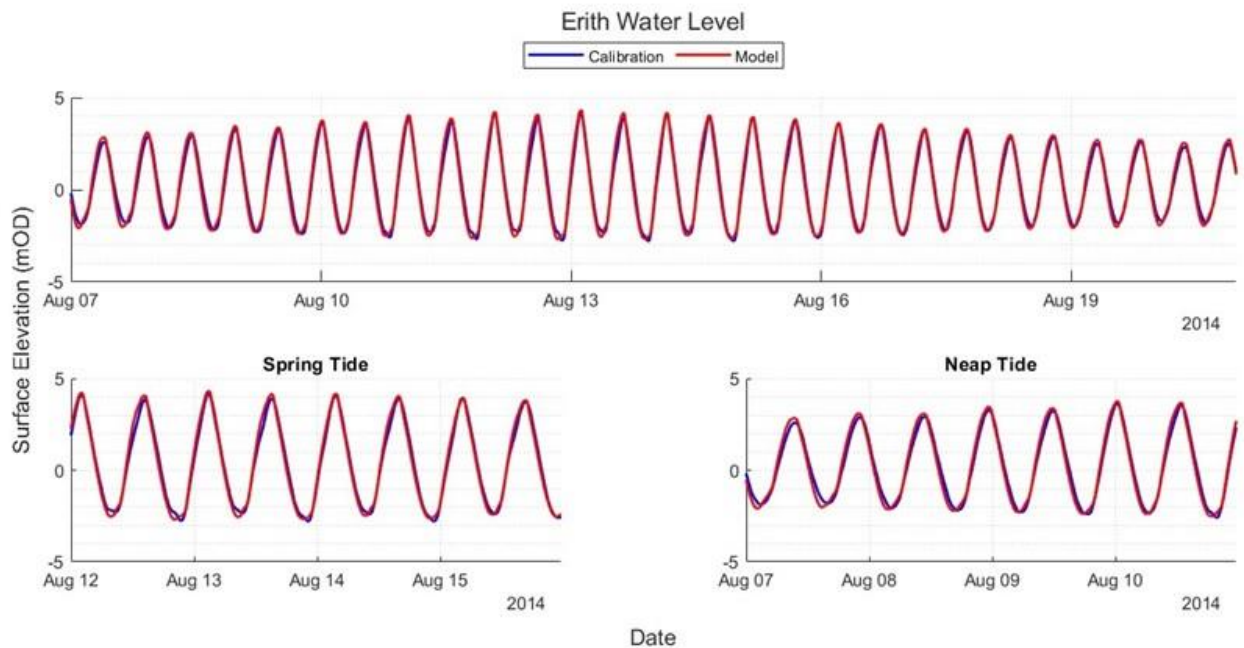
Figure 2-5: Model Surface Elevation (mOD) 2014 Calibration Data at Erith
