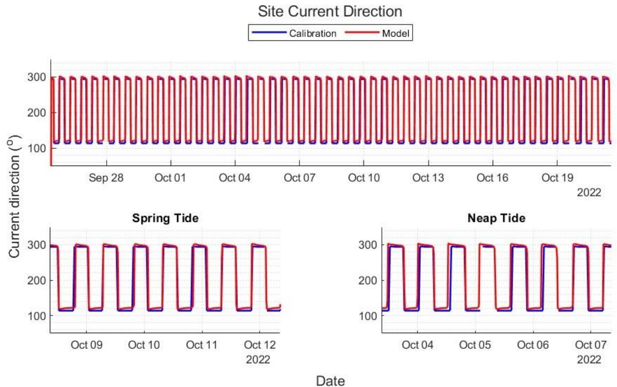
Figure 2-10: Model Current Direction (°) 2022 Validation Data at Station SN011I
